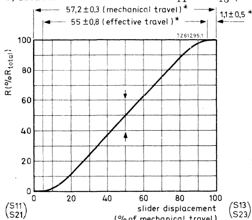
Fig. 9a Linear law; without tap
