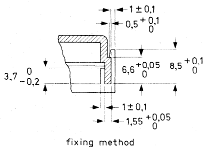
Fig. 5 Method of fixing potentiometer unit 2322 460 90018 e.g. to a tripler unit BG 1897-541.
