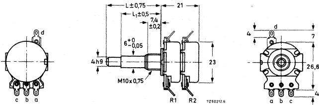
Fig. 3 Twin potentiometer.
