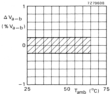
Fig. 6 R_n = 100 \text{ k}\Omega , linear law.
