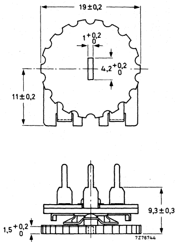
Fig.8 Potentiometer 2322 411 433.. (adjustment wheel at the side of the carbon track).
