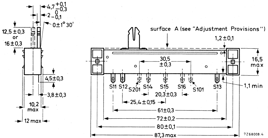
Fig. 1 Single slide potentiometer with solder tags.
