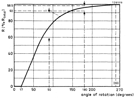
Fig. 9c. Reversed logarithmic resistance law, single potentiometers.
