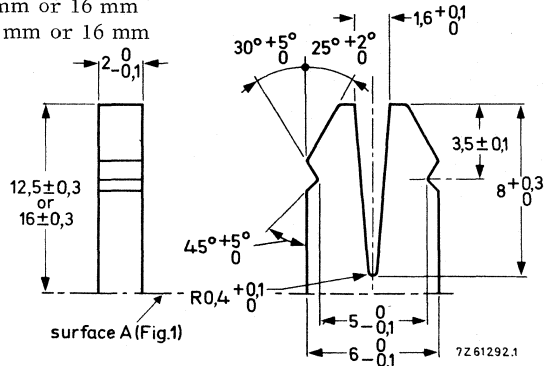
Fig. 8 Adjustment slider.
