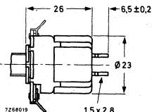
Fig. 9. D.P.S.T. rotary switch (single potentiometer).
