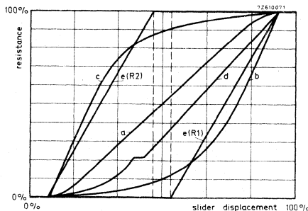
Fig. 2 Resistance laws.
