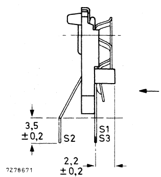
Fig. 5 Test switch for vertical mounting, with two active switch connections; a. with "centre-off" position, b. without "centre-off" position, c. hole pattern for mounting on a printed-wiring board (solder side).
