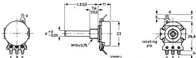
Fig. 1a Single potentiometer with mounting bushing.
