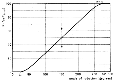
Fig. 3. Resistance as a function of the angle of rotation.
