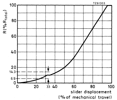
Fig. 9p Semi-logarithmic law; tap at 1/3.
