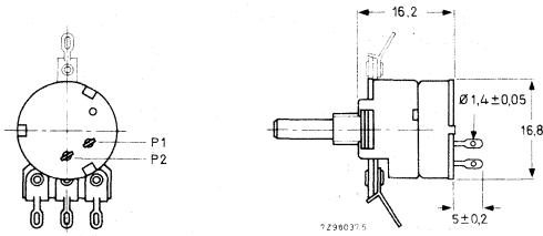
Fig. 4b Single potentiometer with s.p.s.t. rotary switch (spring actuated).
