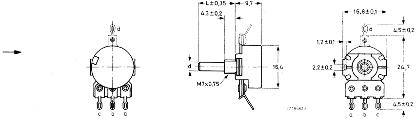
Fig. 1 Single potentiometer with mounting bushing. For dimensions d and L, see Spindles.
