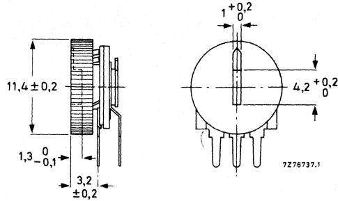
Fig.4 Potentiometer for vertical mounting with knob 2322 410 611 . .
