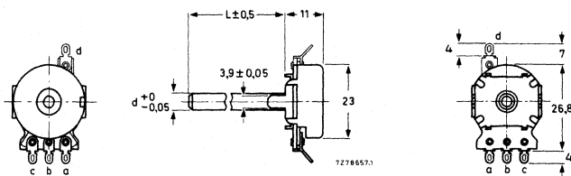
Fig. 1b Single potentiometer with twist tags.
