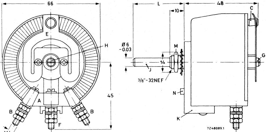
Fig. 3. Potentiometers 2322 097 .....; 0.75 \Omega to 10 k \Omega , 100 W
