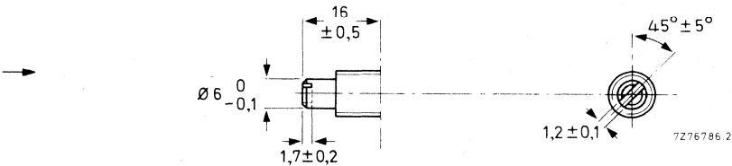
Fig.1b Spindle with screwdriver slot; spindle fully counter clockwise.
