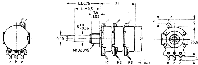
Fig. 4 Triple potentiometer.
