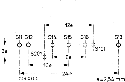
Fig. 5 Hole pattern of the printed-wiring board for a single potentiometer (viewed on component side).
