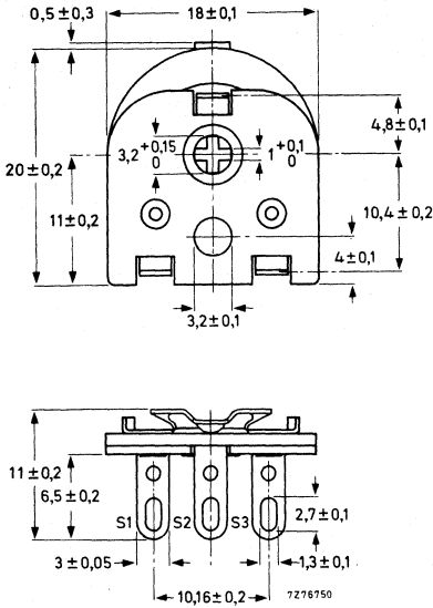
Fig.1 Potentiometer 2322 411 000..
