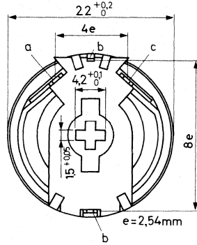
Fig.1 Non-tapped potentiometer without knob.
