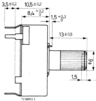
Fig.2 Tapped potentiometer with knob.
