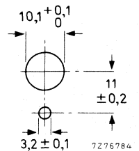
Fig.2 Mounting holes.
