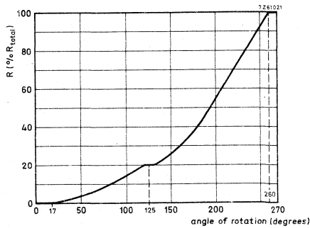
Fig. 9e. Resistance law, tap at 20%, single potentiometers.
