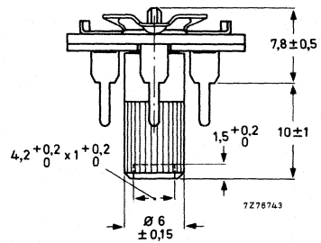
Fig.9 Potentiometer 2322 411 133.. (adjustment knob * at the side of the base plate).
