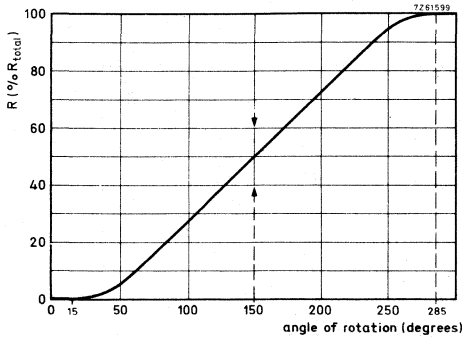
Fig. 10a. Linear resistance law, tandem potentiometers.
