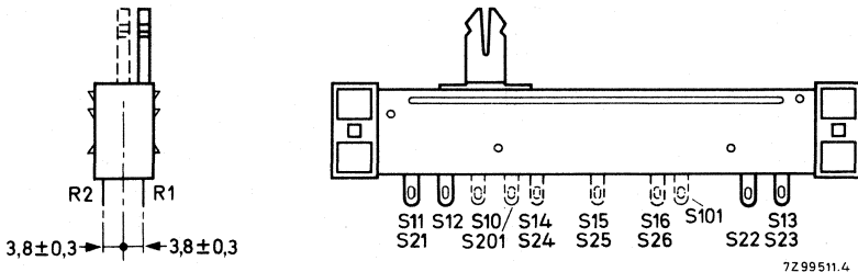
Fig. 2 Tandem slide potentiometer with solder tags.
