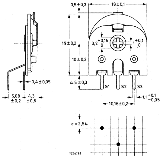
Fig.3 Potentiometer 2322 411 072..
