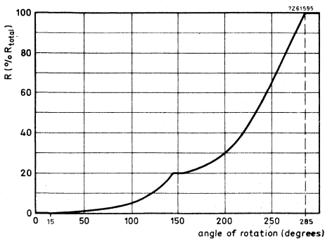
Fig. 10e. Resistance law, tap at 20%, tandem potentiometers.
