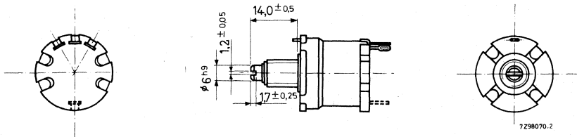
Fig. 4. Potentiometers 2322 010 . . . . with spindle with screwdriver slot. Dimensions are identical to those in Fig. 3. except as shown.
