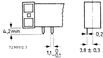
Fig. 4 Printed-wiring pins.
