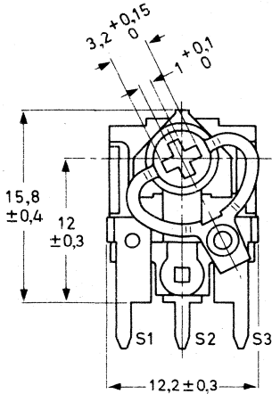
Fig. 4 Test switch for horizontal mounting with adjustment knob at the side of the base plate.
