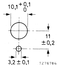
Fig. 2 Mounting holes.
