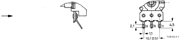
Fig.5 Solder tags.
