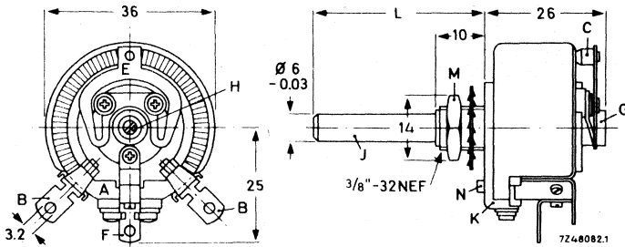
Fig.1. Potentiometers 2322 095 ..... ; 1 Ω to 7.5 kΩ, 25 W
