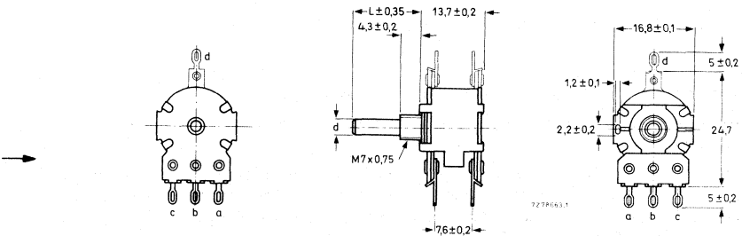
Fig. 3 Tandem potentiometer. For dimensions d and L, see Spindles.
