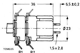
Fig. 10. D.P.S.T. rotary switch (tandem or twin potentiometer).
