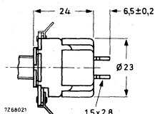
Fig. 11. D.P.S.T. push-pull switch (single potentiometer).
