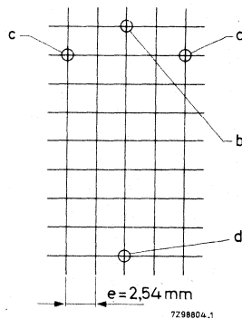
Fig.4 Mounting holes for tapped potentiometers.
