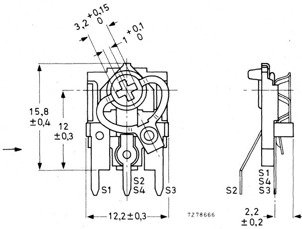
Fig. 6a Test switch for vertical mounting, with three active switch conditions.
