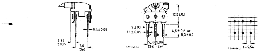
Fig. 7 Long or short printed-wiring pins (tandem potentiometer).
