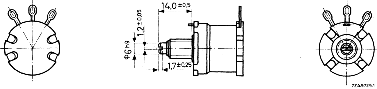
Fig. 2. Potentiometers 2322 003 . . . . with spindle with screwdriver slot. Dimensions are identical to those in Fig. 1. except as shown.
