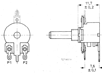
Fig. 4c Single potentiometer with s.p.s.t. rotary switch (direct operating).
